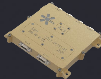
ADCS control unit
