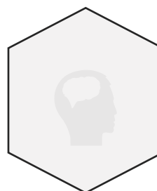
Augmented Intelligence
